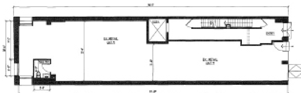
FIRST FLOOR PLAN SCALE 1/8" = 1'-0"
