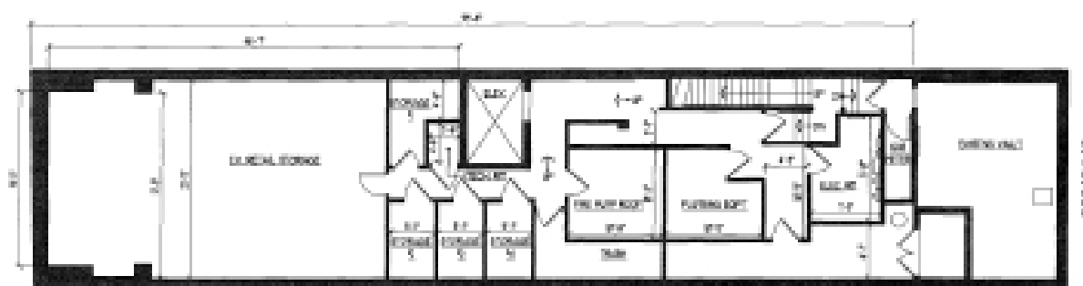
CELLAR FLOOR PLAN SCALE 1/8" = 1'-0"
